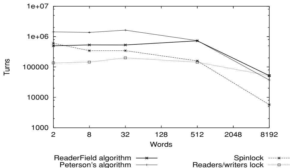
(a) 16 threads, high contention.
