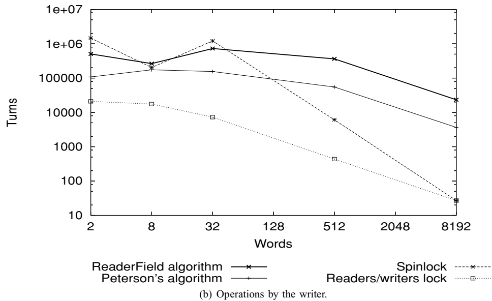
Fig. 6. Average number of operations per thread with 14 threads and high contention on NUMA Origin 2000.
