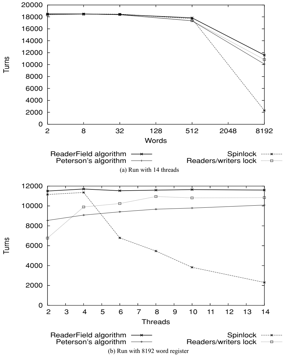
Fig. 8. Average number of operations per thread with low contention on NUMA Origin 2000.
