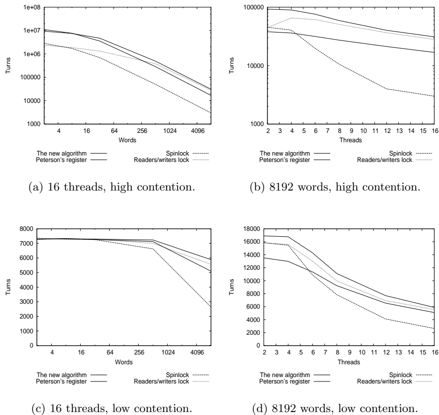
Fig. 5. Average number of reads or writes per process on the UMA SunFire 880.
