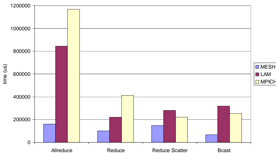
Figure 5: Collective Operations latencies from Pallas 4MB messages.
