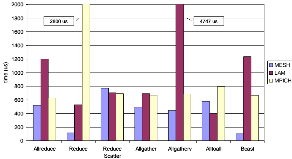
Figure 4: Collective Operations latencies from Pallas 8B messages.
